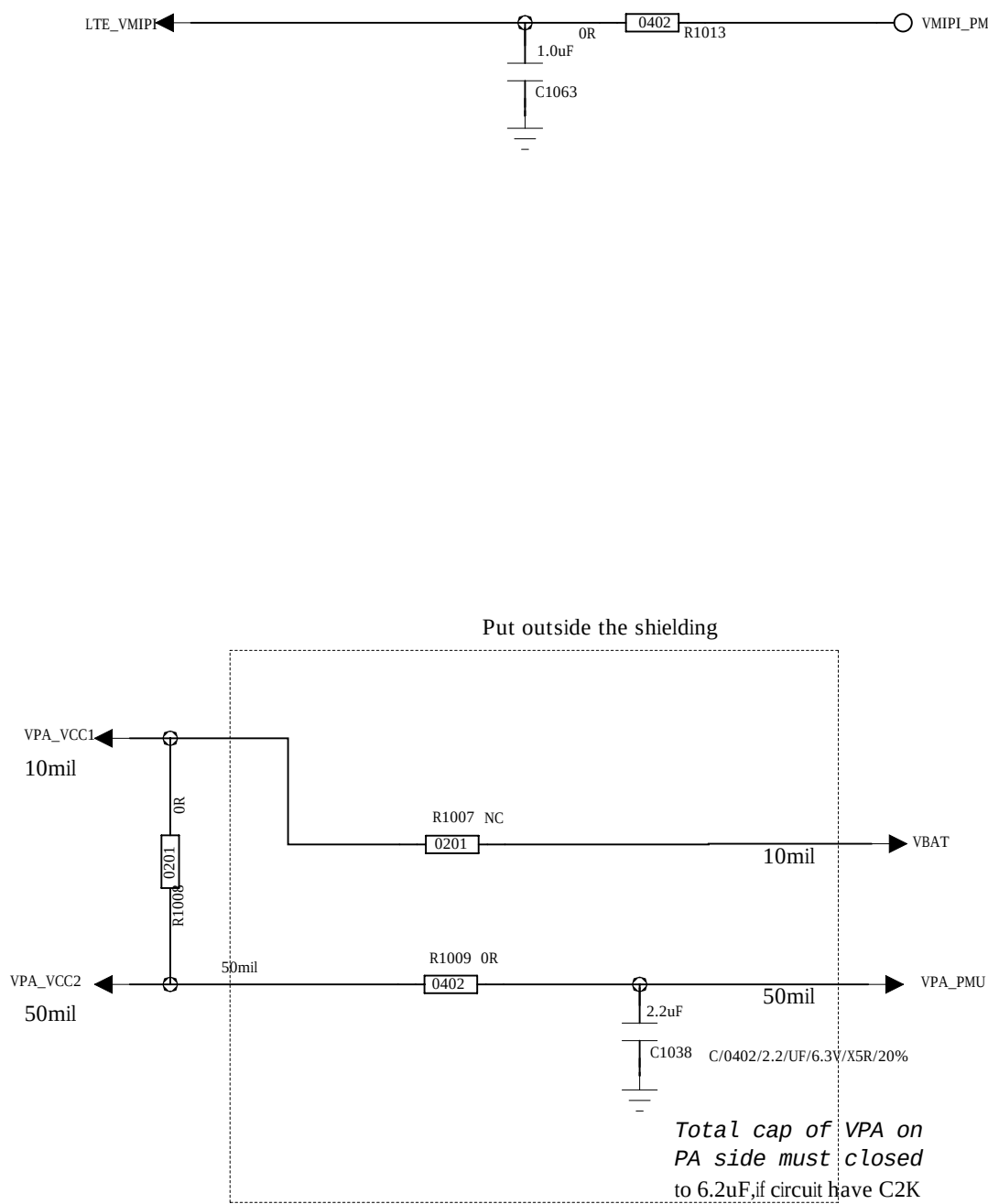
Power Net Connection
